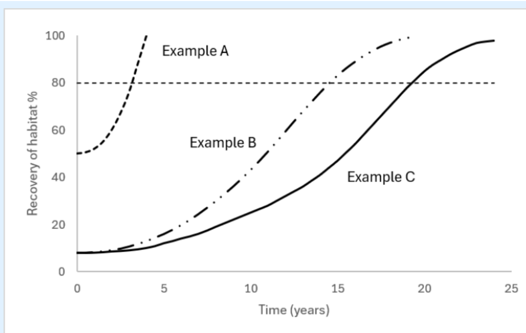
Figure GSA5: Example recovery rates for habitats over time under different fishing conditions where fishing is removed at year 0
